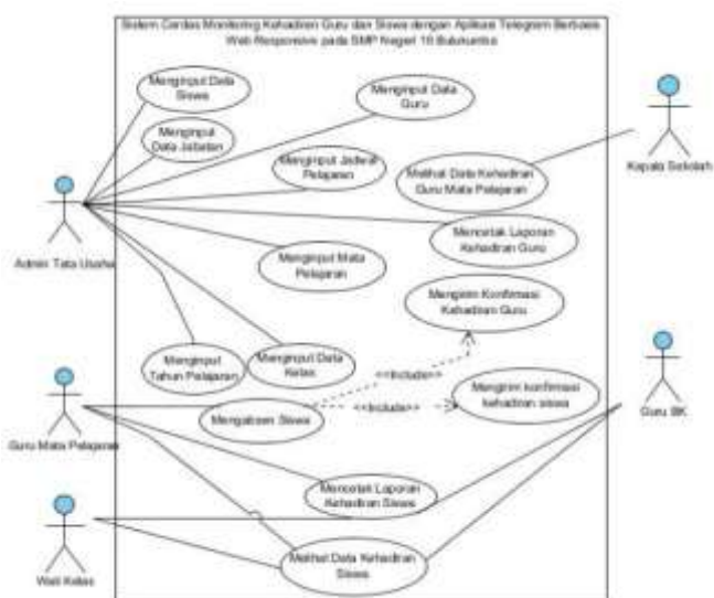
Gambar 3.2. Use Case Diagram Sistem cerdas monitoring
