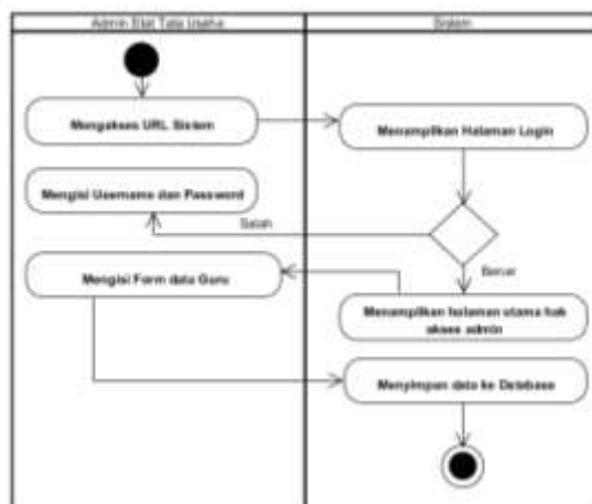
Gambar 3.3. Activity Diagram Input Data Guru
