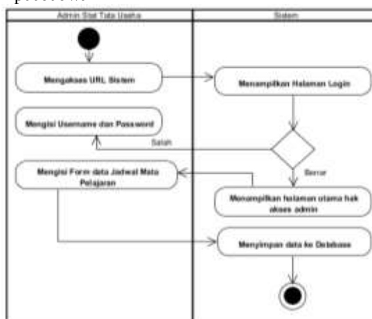
Gambar 3.5. Activity Diagram Input Jadwal
